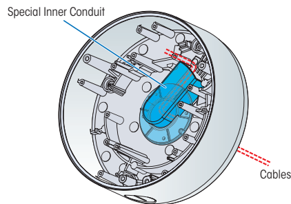
Water-resistant Design (SNC-DF85/DF80 inside)
