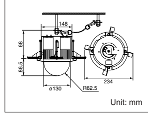
Suspended Ceiling Installation WV-Q117
