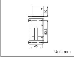
Suspended Ceiling Installation WV-Q107A
